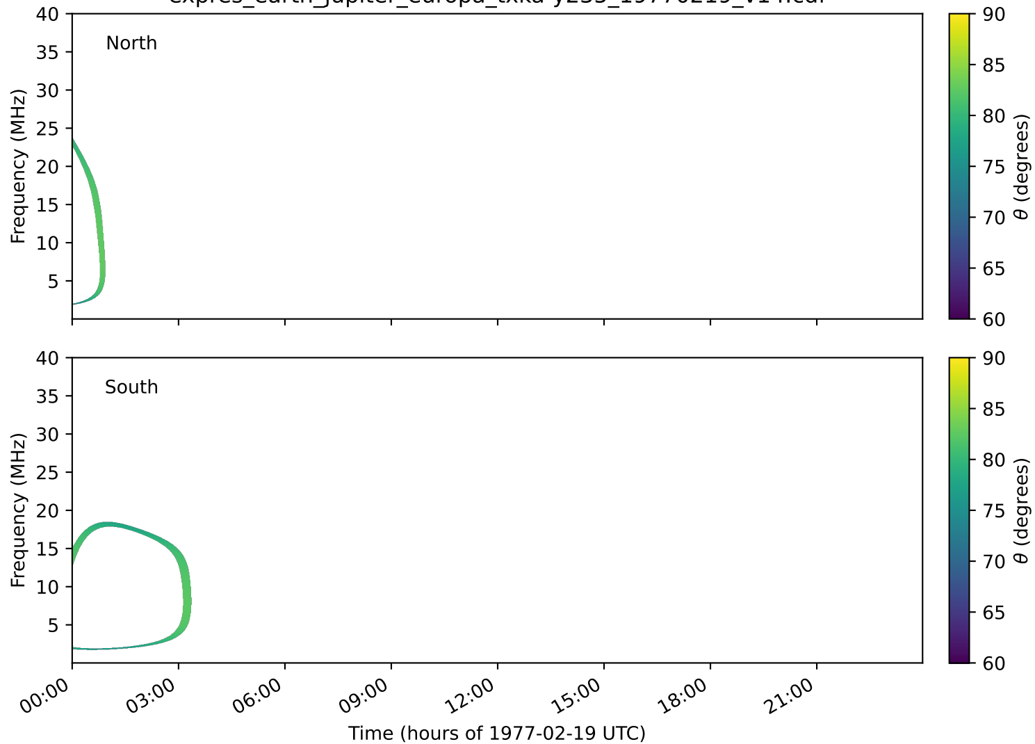
expres_earth_jupiter_europa_txka-y235_19770219_v14.cdf
