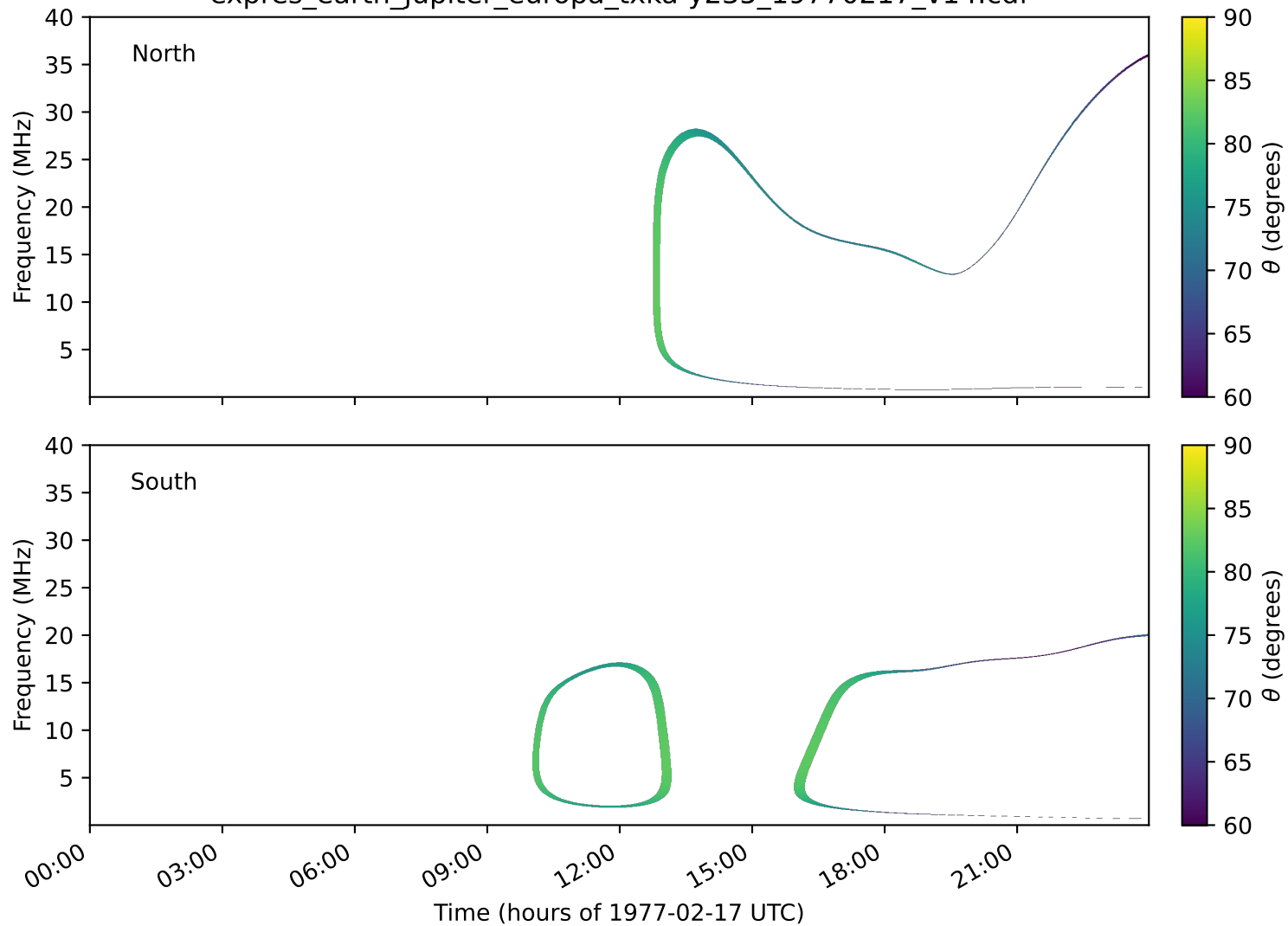
expres_earth_jupiter_europa_txka-y235_19770217_v14.cdf
