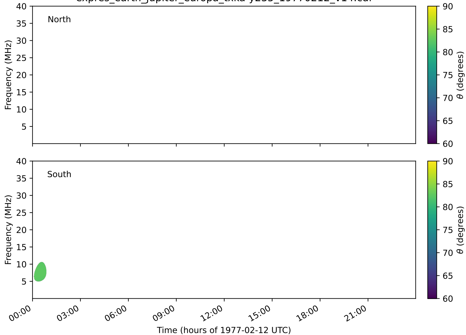
expres_earth_jupiter_europa_txka-y235_19770212_v14.cdf
