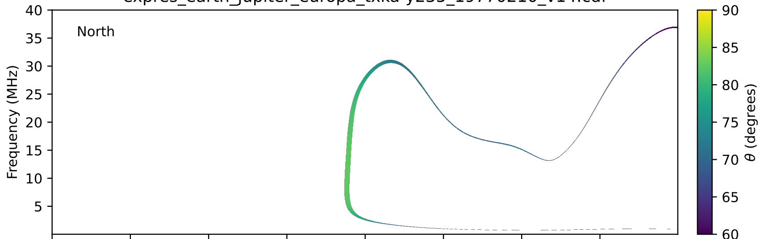
expres_earth_jupiter_europa_txka-y235_19770210_v14.cdf
