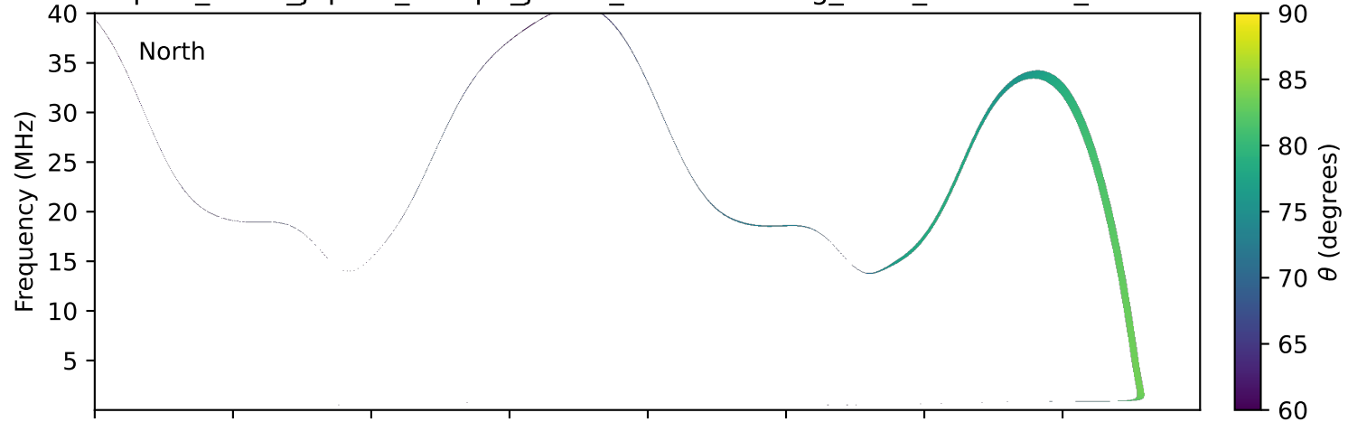
expres_earth_jupiter_europa_jrm33_lossc-wid1deg_3kev_19770204_v11.cdf
