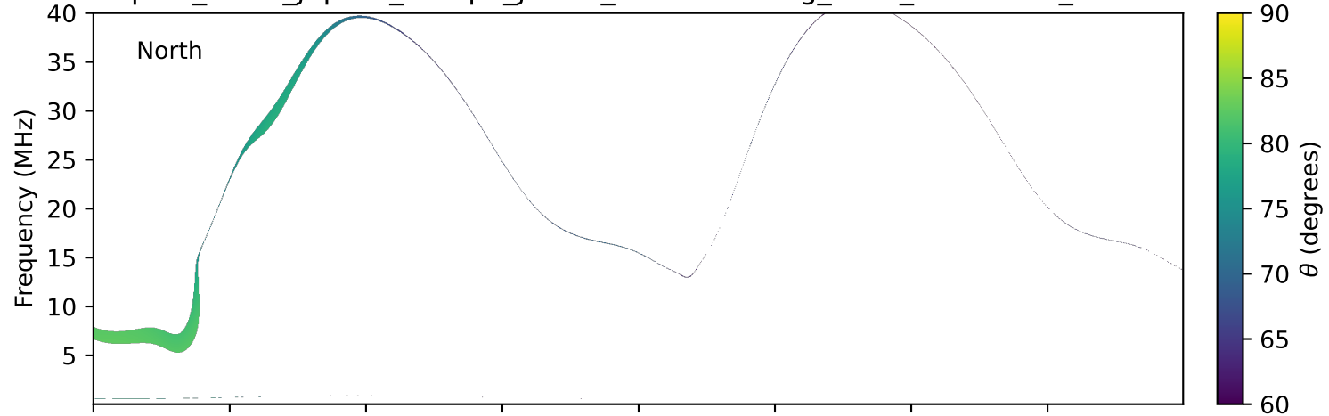
expres_earth_jupiter_europa_jrm09_lossc-wid1deg_3kev_19770214_v11.cdf
