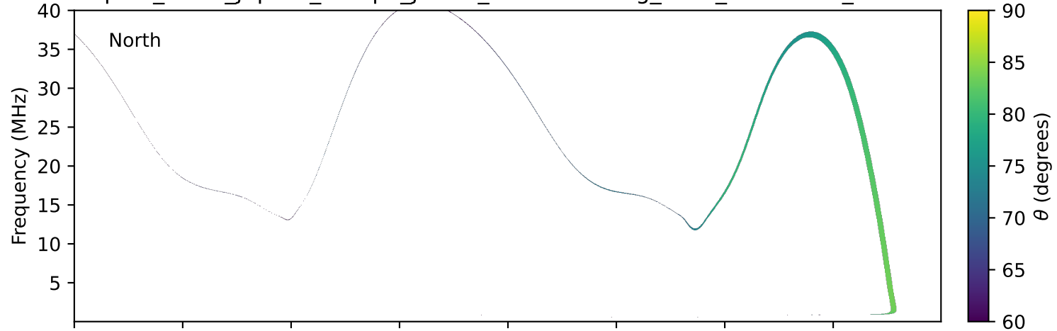
expres_earth_jupiter_europa_jrm09_lossc-wid1deg_3kev_19770204_v11.cdf
