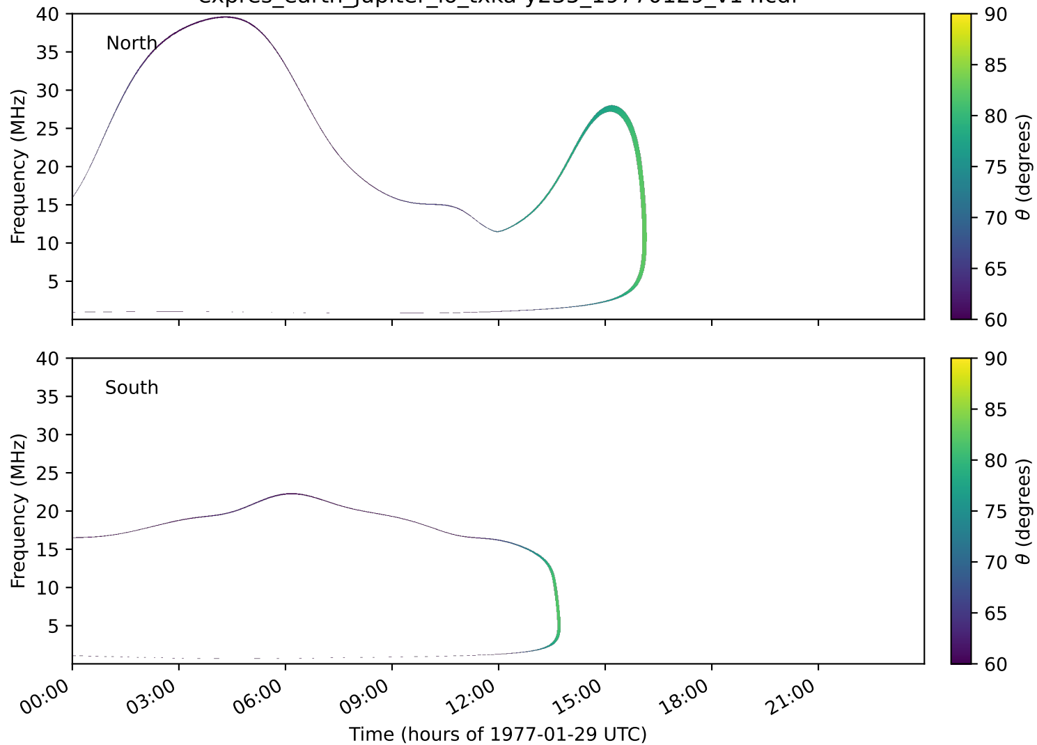
expres_earth_jupiter_io_txka-y235_19770129_v14.cdf
