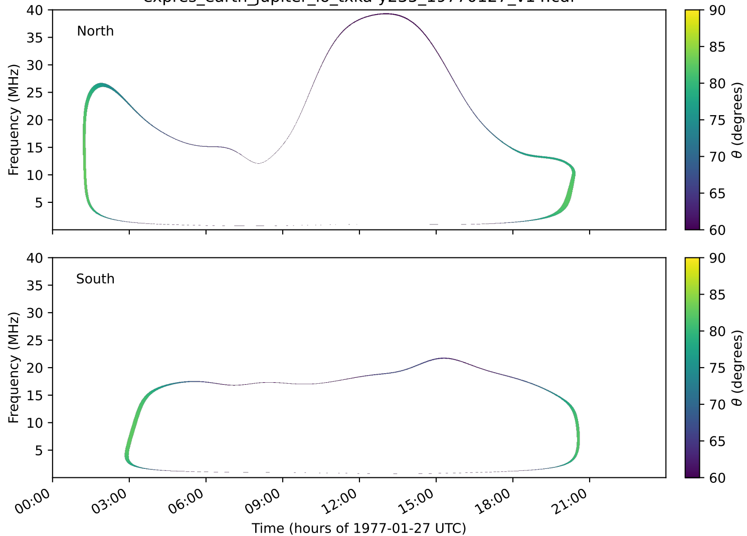
expres_earth_jupiter_io_txka-y235_19770127_v14.cdf
