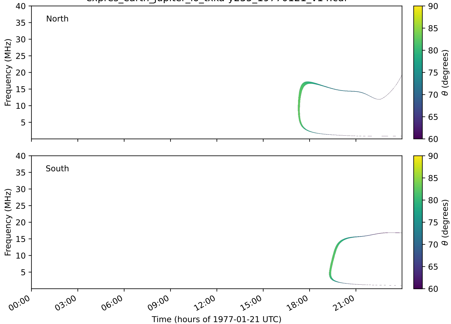
expres_earth_jupiter_io_txka-y235_19770121_v14.cdf
