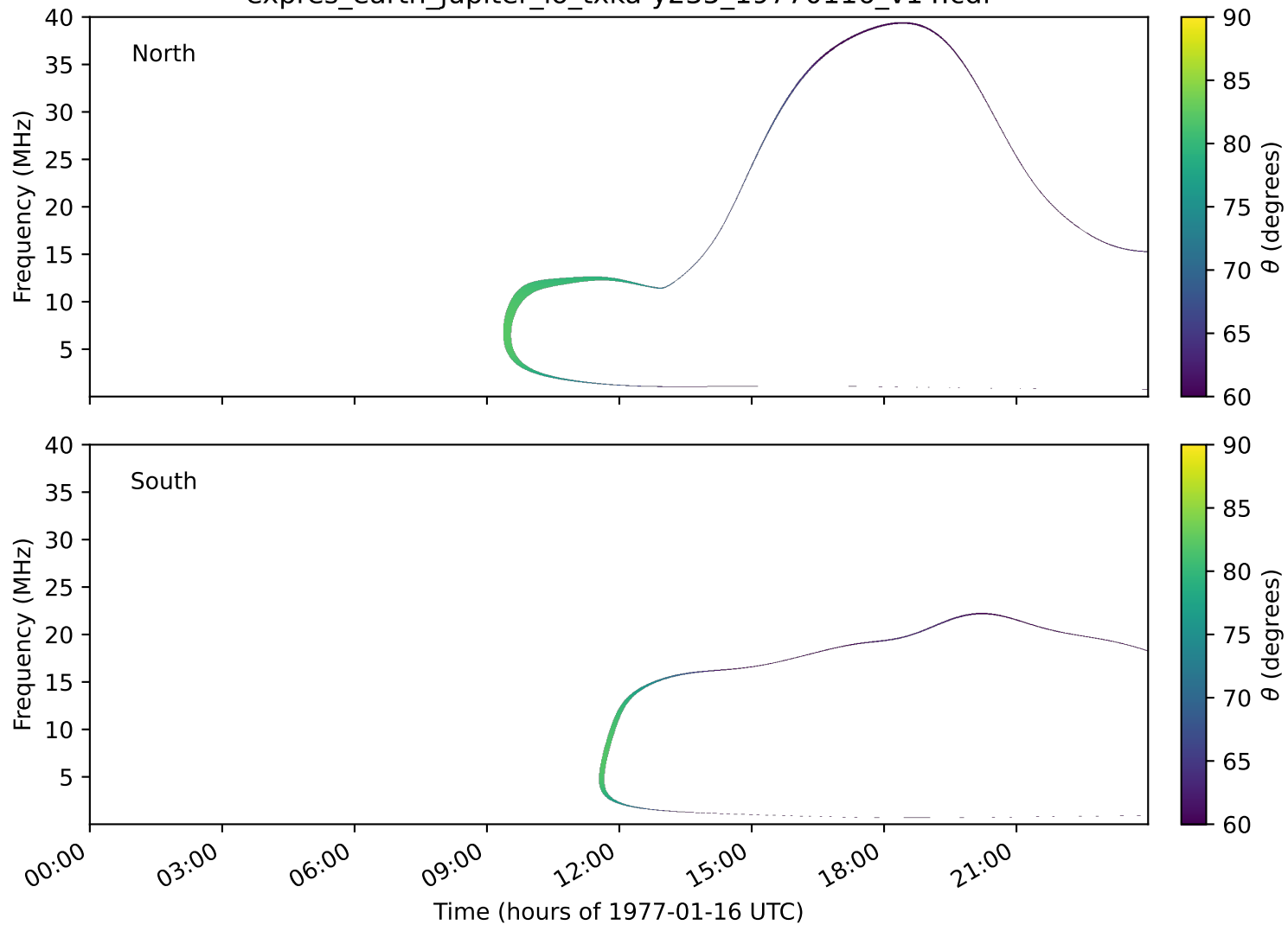
expres_earth_jupiter_io_txka-y235_19770116_v14.cdf
