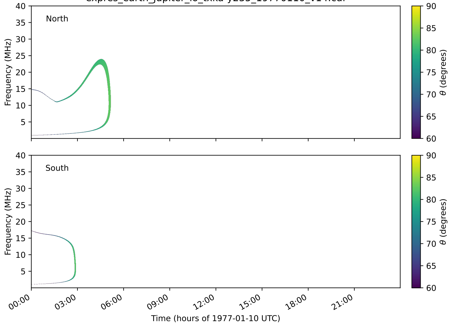
expres_earth_jupiter_io_txka-y235_19770110_v14.cdf
