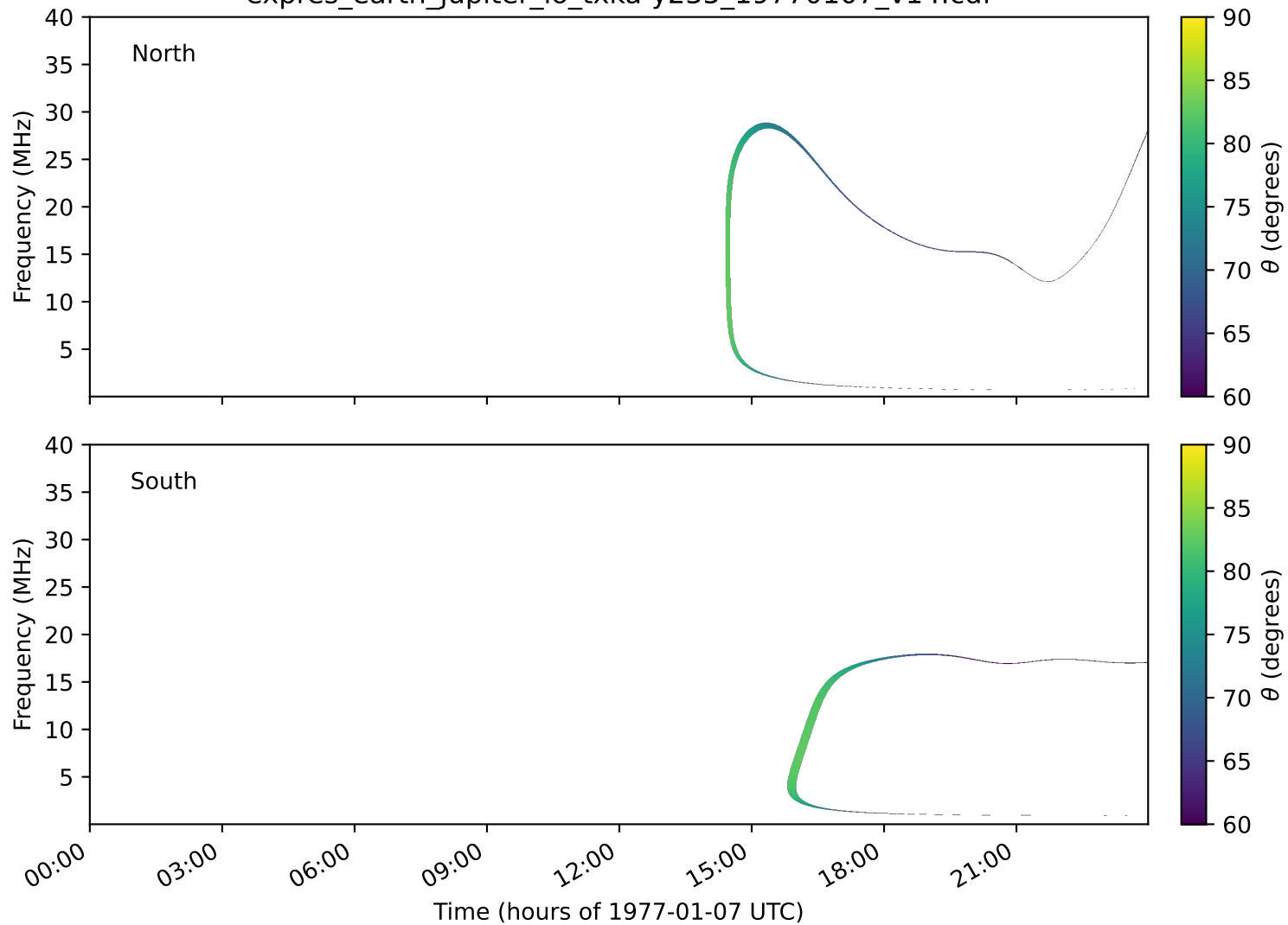
expres_earth_jupiter_io_txka-y235_19770107_v14.cdf
