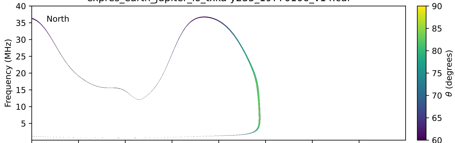
expres_earth_jupiter_io_txka-y235_19770106_v14.cdf
