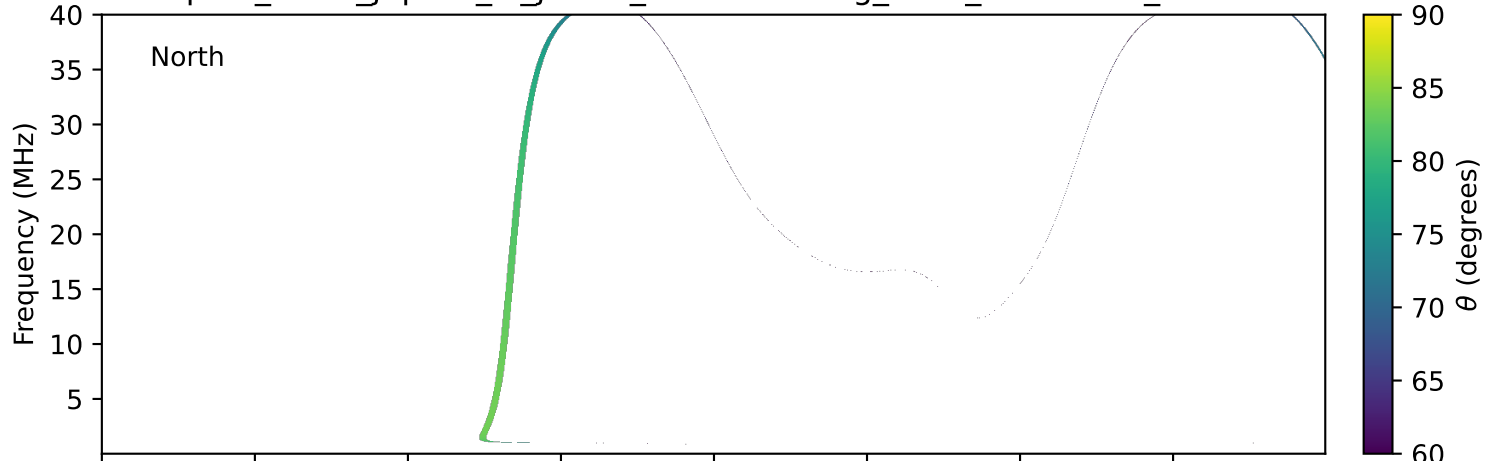
expres_earth_jupiter_io_jrm33_lossc-wid1deg_3kev_19770125_v11.cdf
