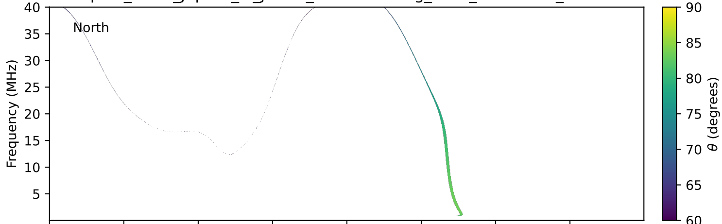
expres_earth_jupiter_io_jrm33_lossc-wid1deg_3kev_19770113_v11.cdf
