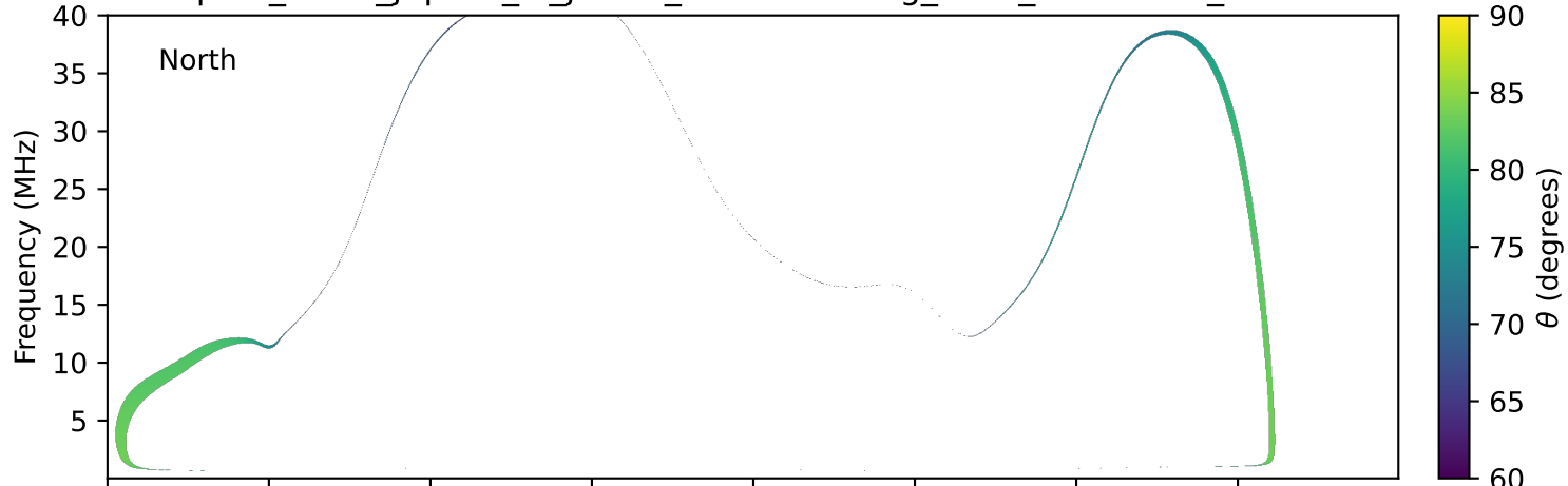
expres_earth_jupiter_io_jrm33_lossc-wid1deg_3kev_19770104_v11.cdf
