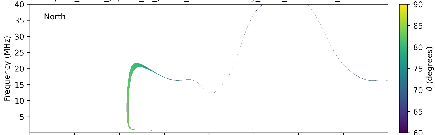
expres_earth_jupiter_io_jrm33_lossc-wid1deg_3kev_19770102_v11.cdf
