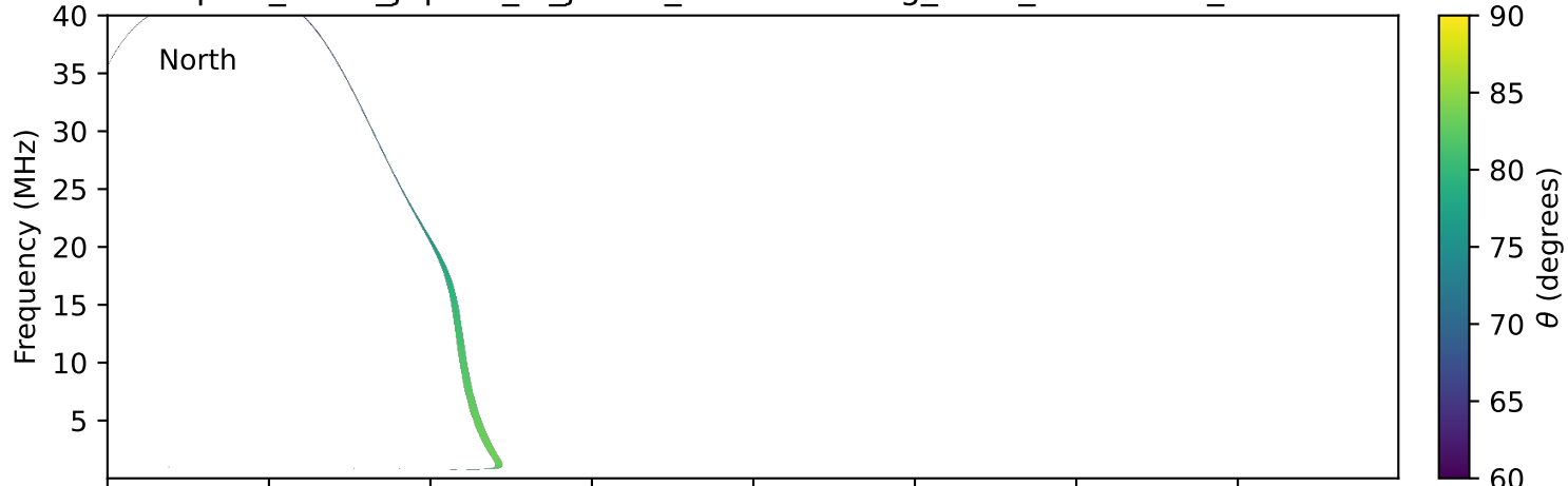
expres_earth_jupiter_io_jrm33_lossc-wid1deg_3kev_19770101_v11.cdf
