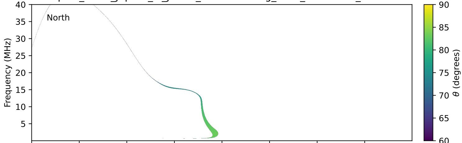
expres_earth_jupiter_io_jrm09_lossc-wid1deg_3kev_19770115_v11.cdf
