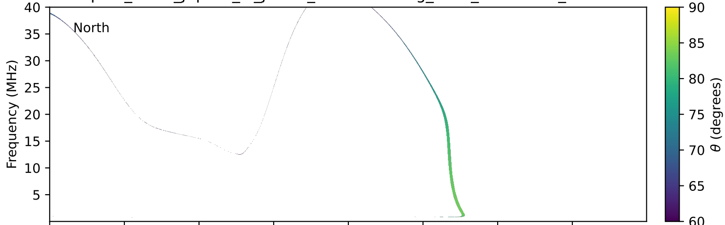
expres_earth_jupiter_io_jrm09_lossc-wid1deg_3kev_19770113_v11.cdf
