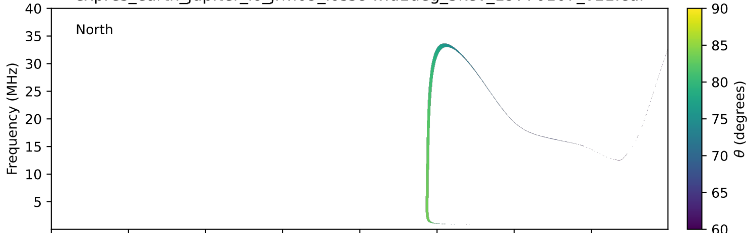
expres_earth_jupiter_io_jrm09_lossc-wid1deg_3kev_19770107_v11.cdf
