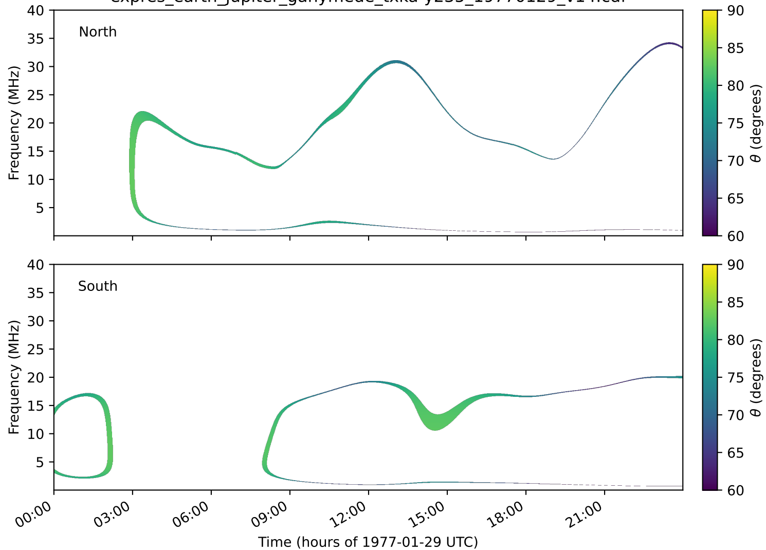
expres_earth_jupiter_ganymede_txka-y235_19770129_v14.cdf
