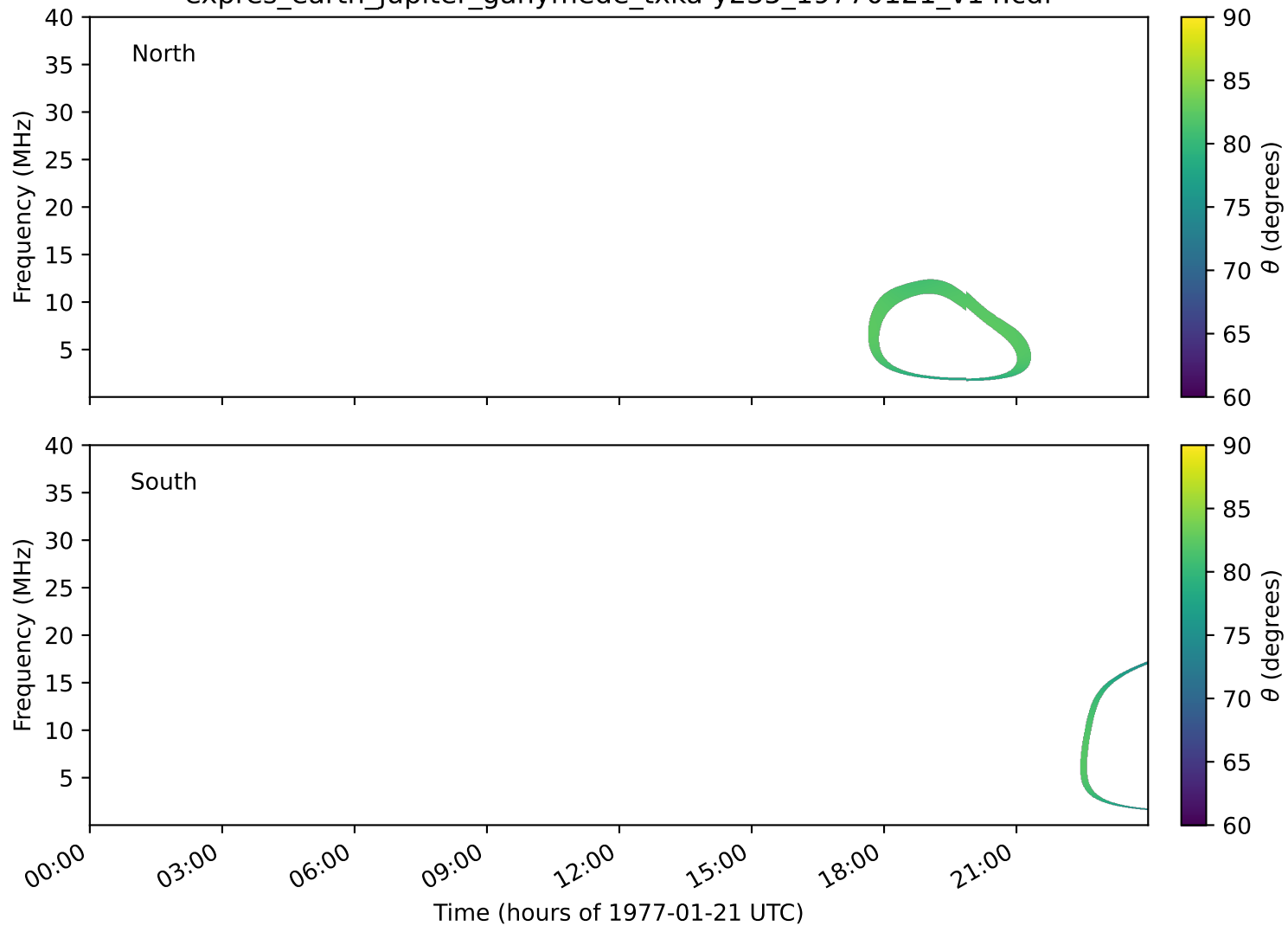
expres_earth_jupiter_ganymede_txka-y235_19770121_v14.cdf
