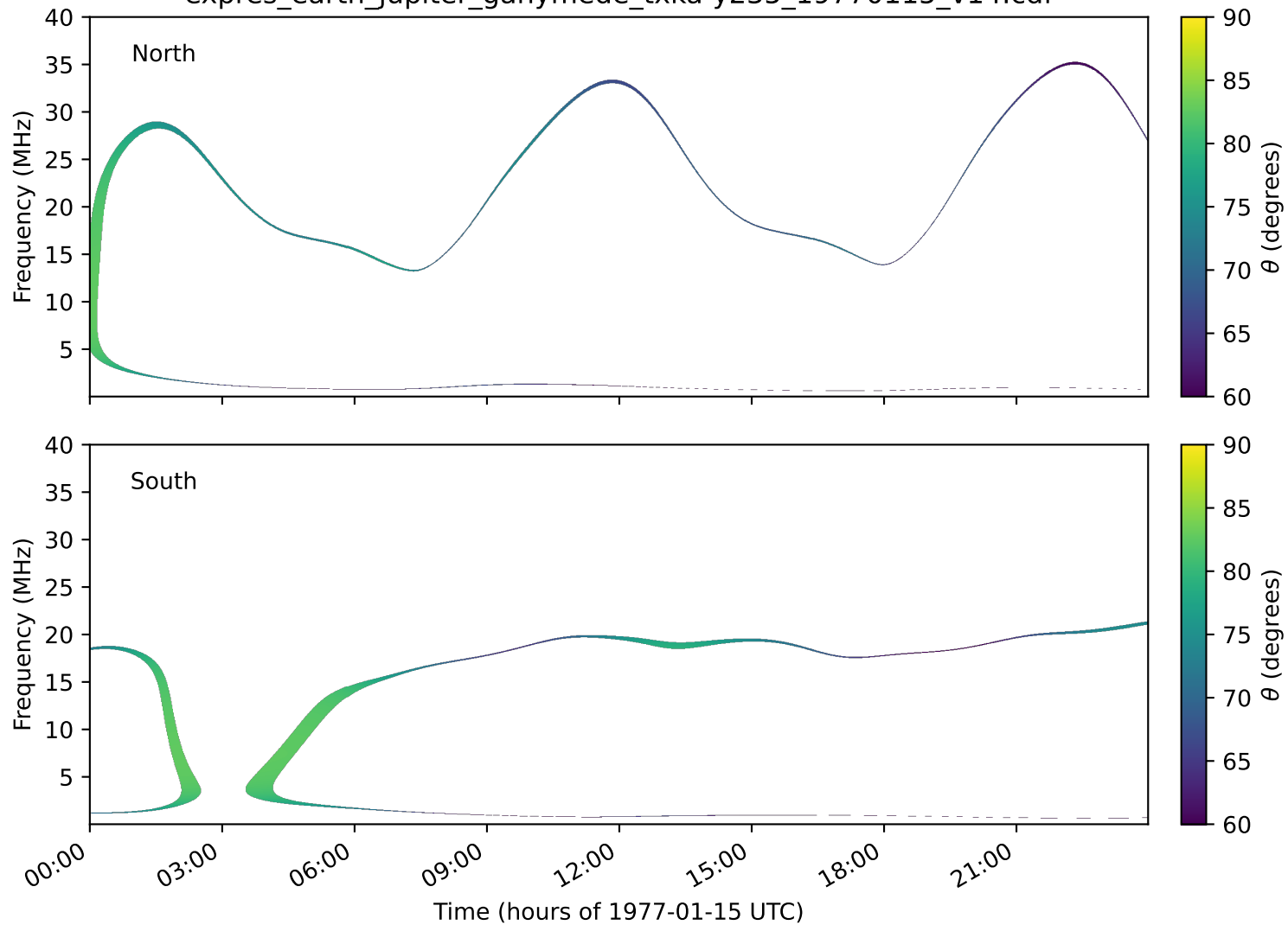
expres_earth_jupiter_ganymede_txka-y235_19770115_v14.cdf
