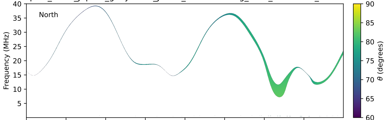
expres_earth_jupiter_ganymede_jrm33_lossc-wid1deg_3kev_19770110_v11.cdf
