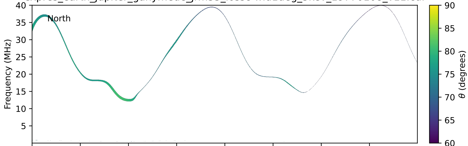
expres_earth_jupiter_ganymede_jrm33_lossc-wid1deg_3kev_19770108_v11.cdf
