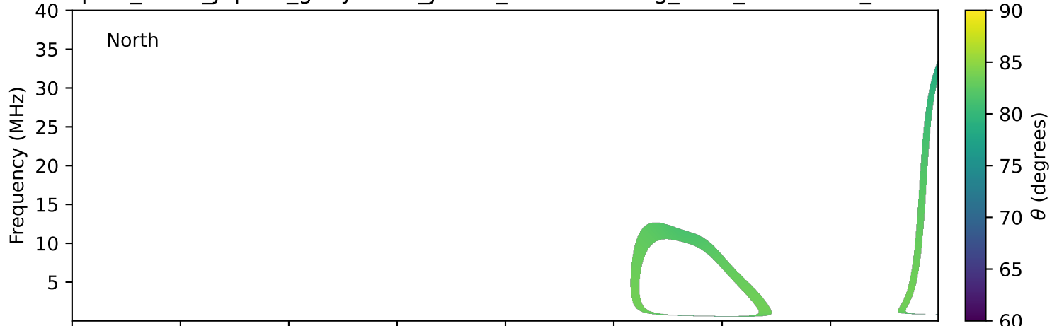
expres_earth_jupiter_ganymede_jrm33_lossc-wid1deg_3kev_19770107_v11.cdf
