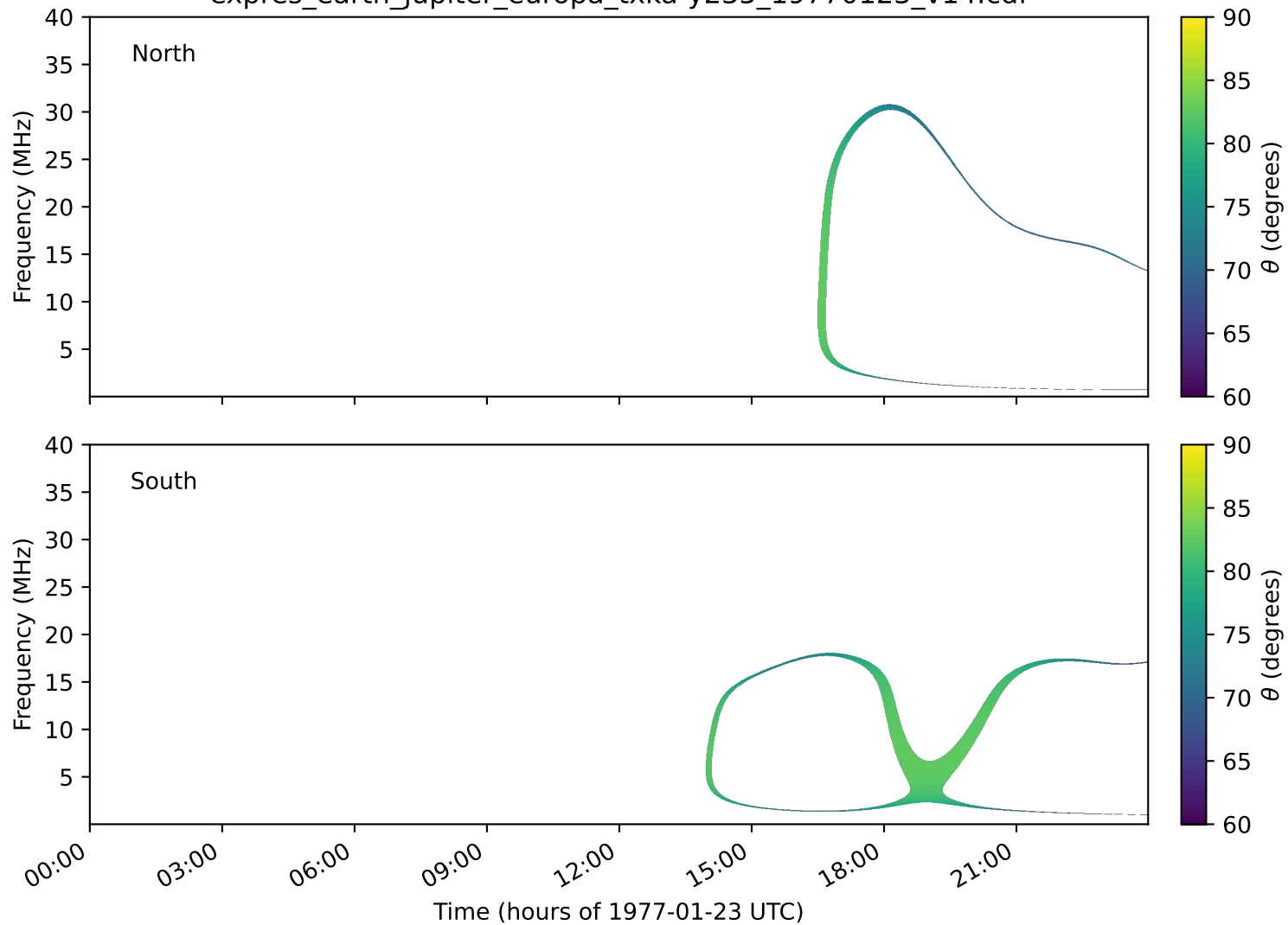
expres_earth_jupiter_europa_txka-y235_19770123_v14.cdf
