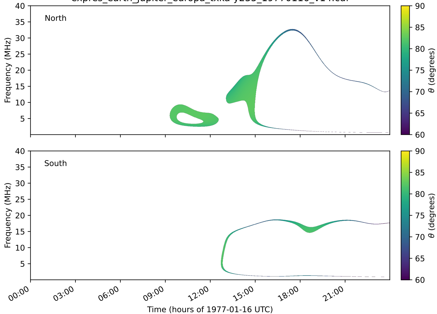
expres_earth_jupiter_europa_txka-y235_19770116_v14.cdf
