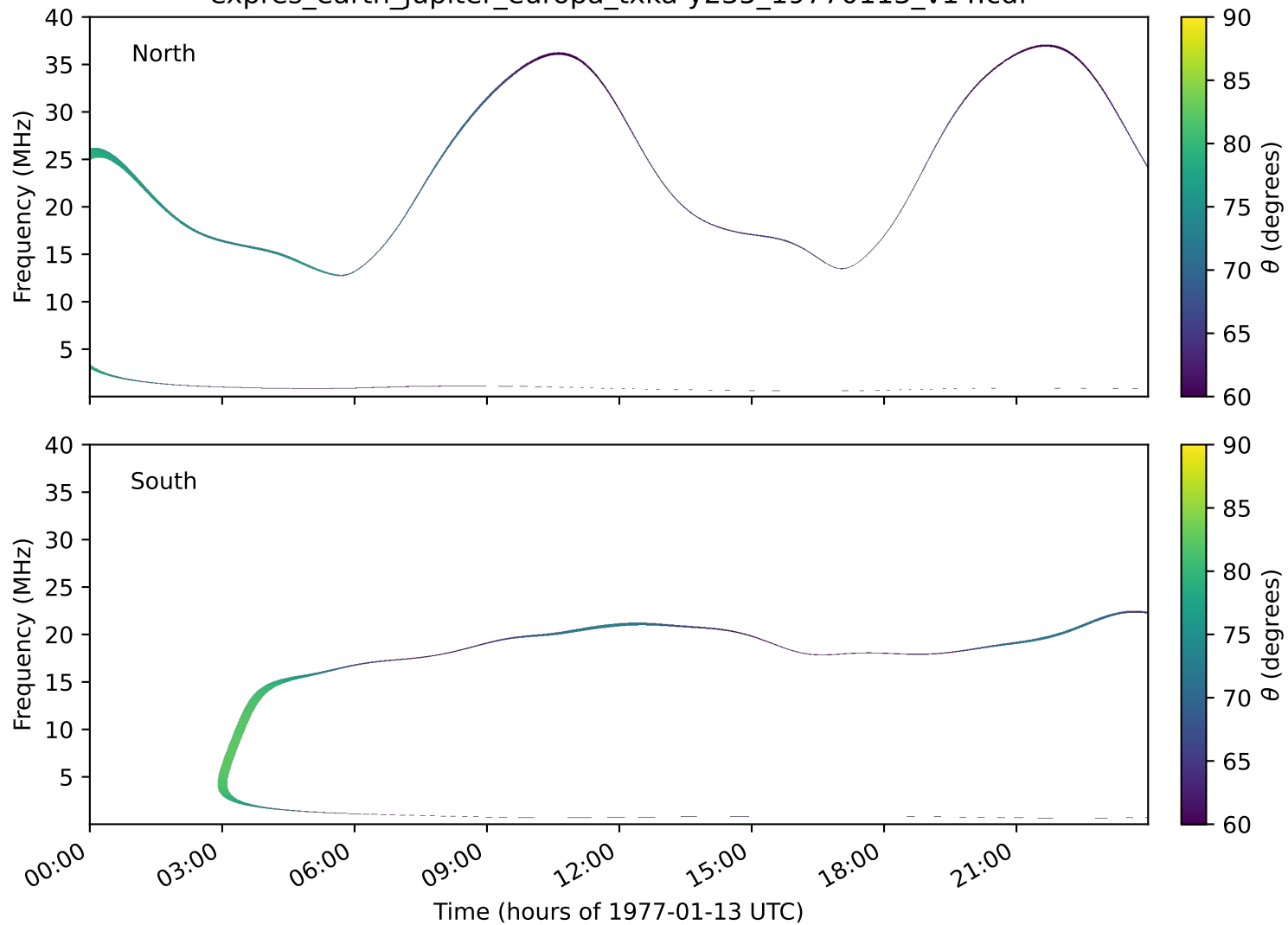
expres_earth_jupiter_europa_txka-y235_19770113_v14.cdf
