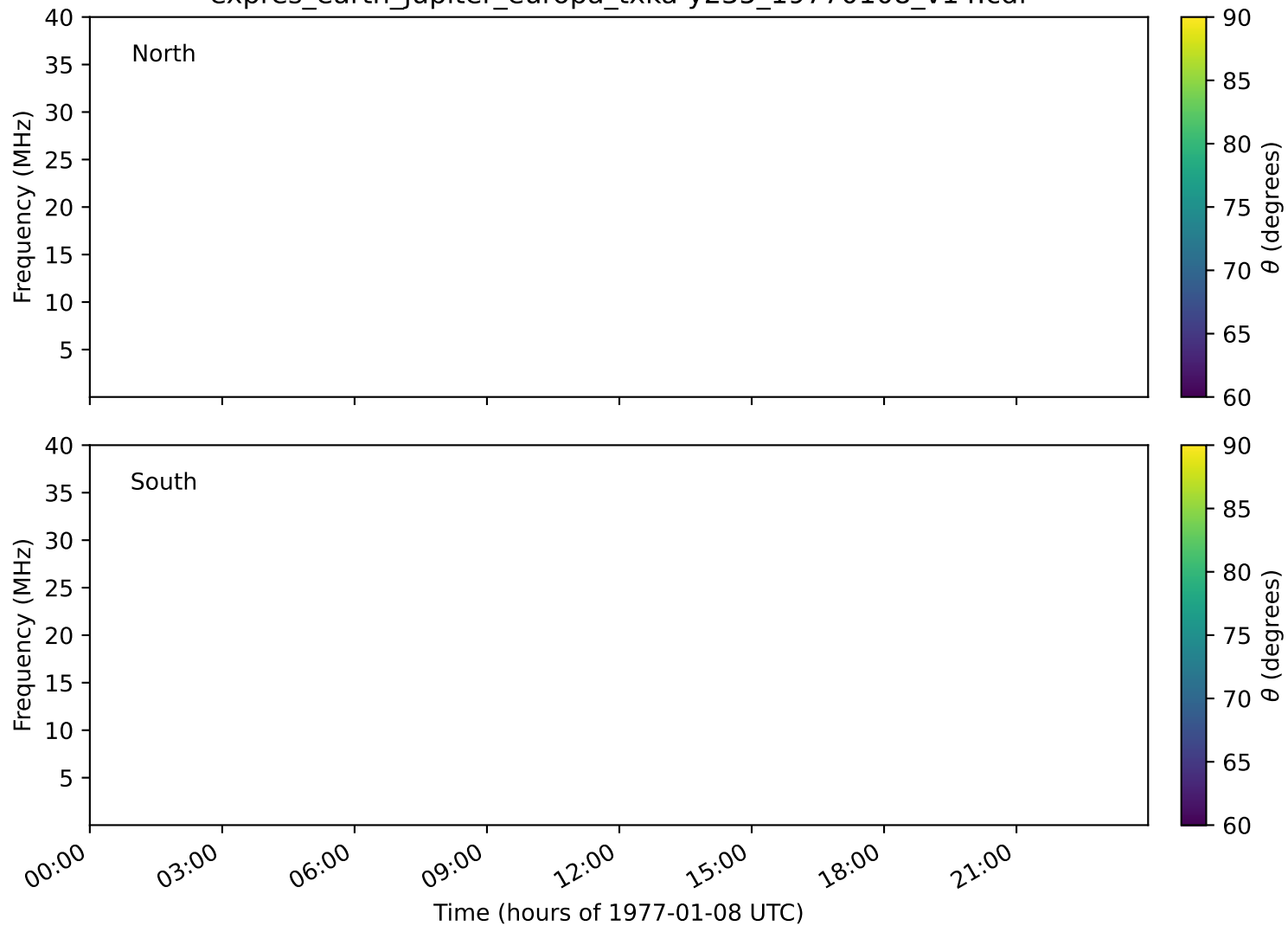
expres_earth_jupiter_europa_txka-y235_19770108_v14.cdf
