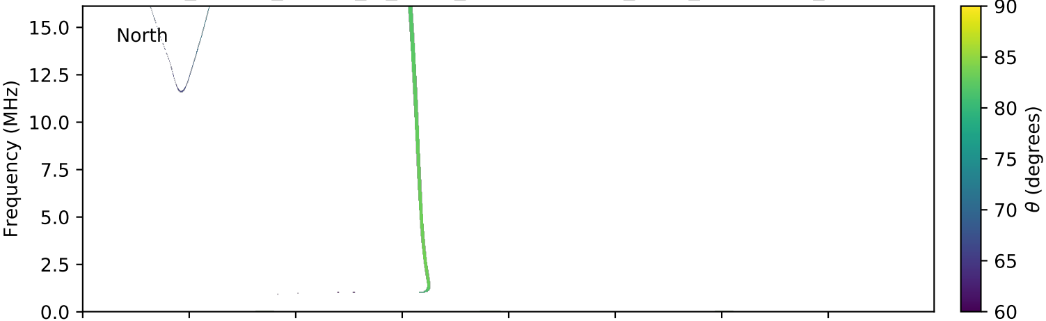
expres_cassini_jupiter_io_isaac_lossc-wid1deg_3kev_20020629_v01.cdf
