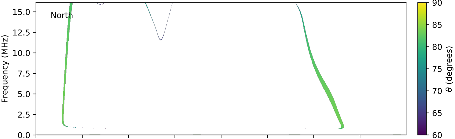
expres_cassini_jupiter_io_isaac_lossc-wid1deg_3kev_20020625_v01.cdf
