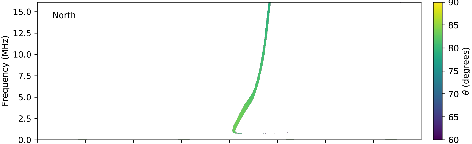
expres_cassini_jupiter_io_isaac_lossc-wid1deg_3kev_20020621_v01.cdf
