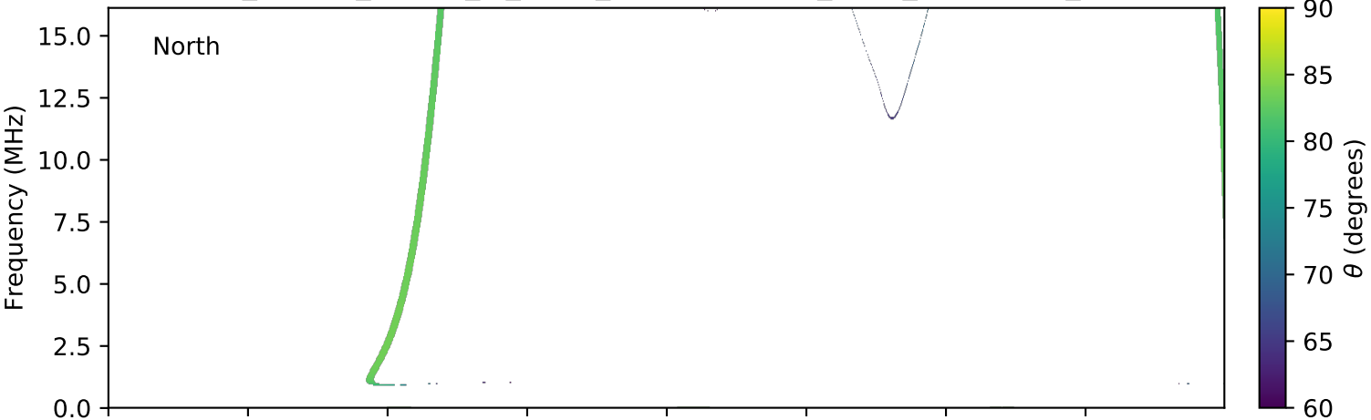
expres_cassini_jupiter_io_isaac_lossc-wid1deg_3kev_20020616_v01.cdf
