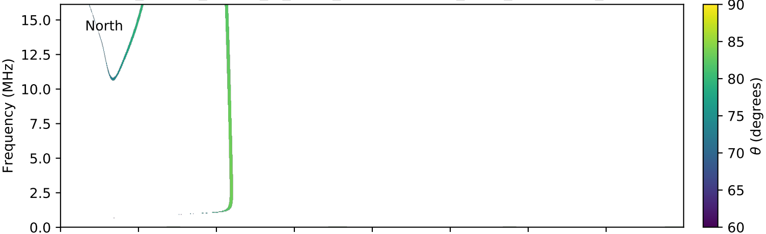
expres_cassini_jupiter_io_isaac_lossc-wid1deg_3kev_20020615_v01.cdf
