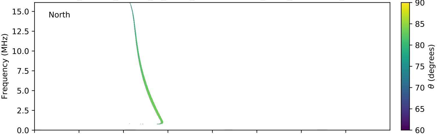
expres_cassini_jupiter_io_isaac_lossc-wid1deg_3kev_20020606_v01.cdf
