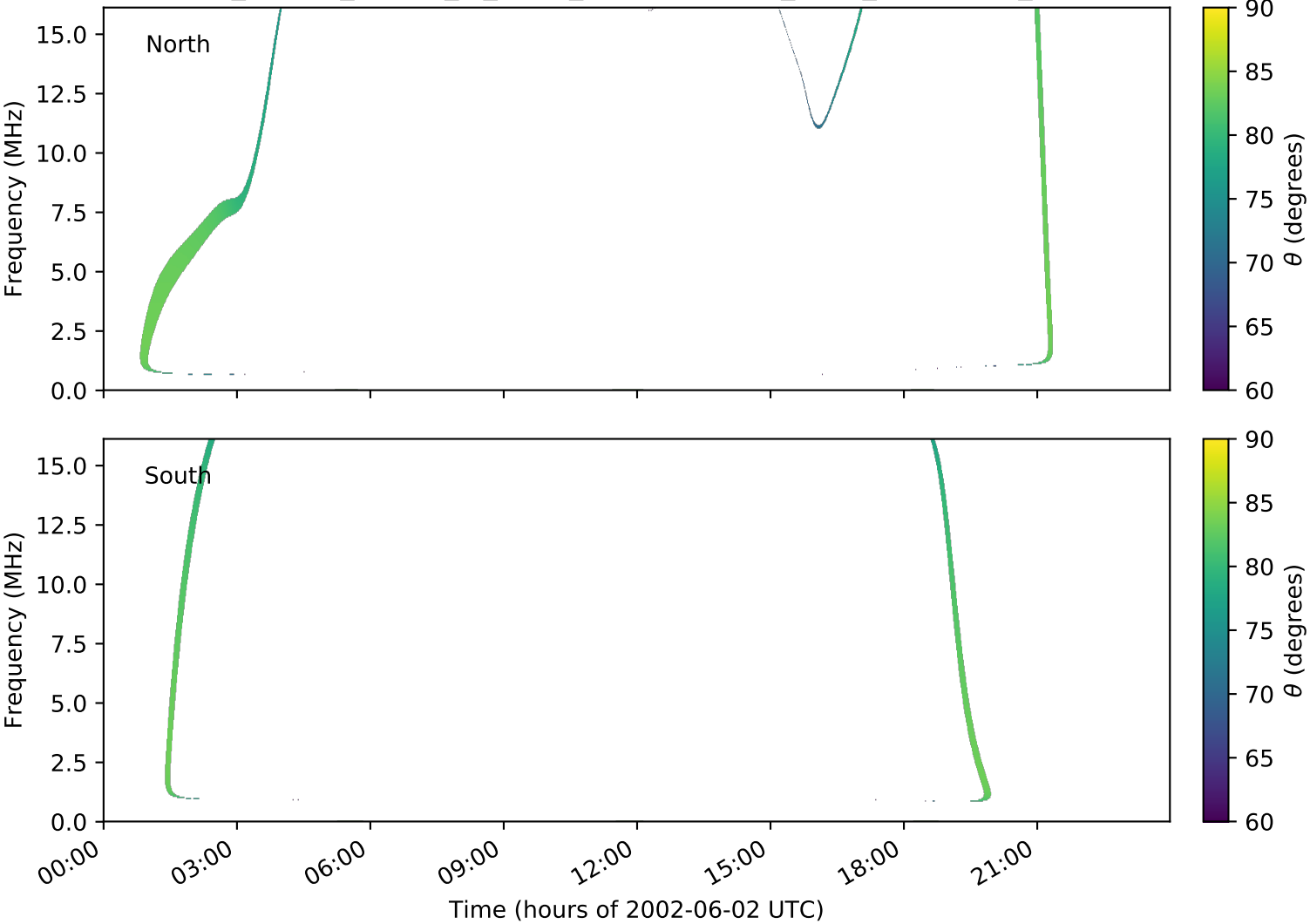
expres_cassini_jupiter_io_isaac_lossc-wid1deg_3kev_20020602_v01.cdf
