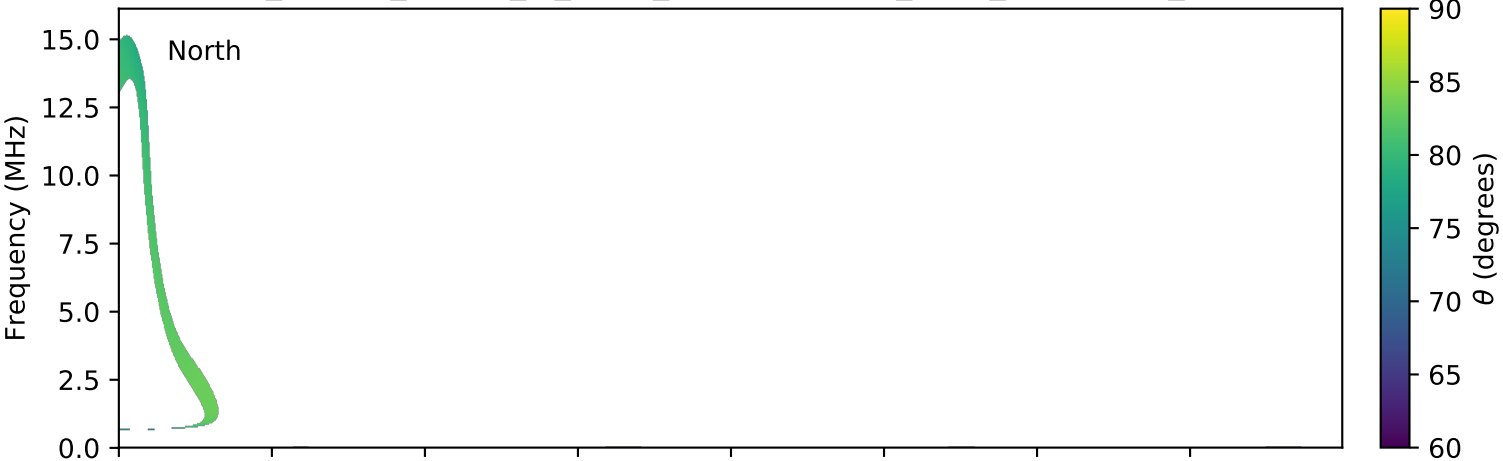
expres_cassini_jupiter_io_isaac_lossc-wid1deg_3kev_20020601_v01.cdf
