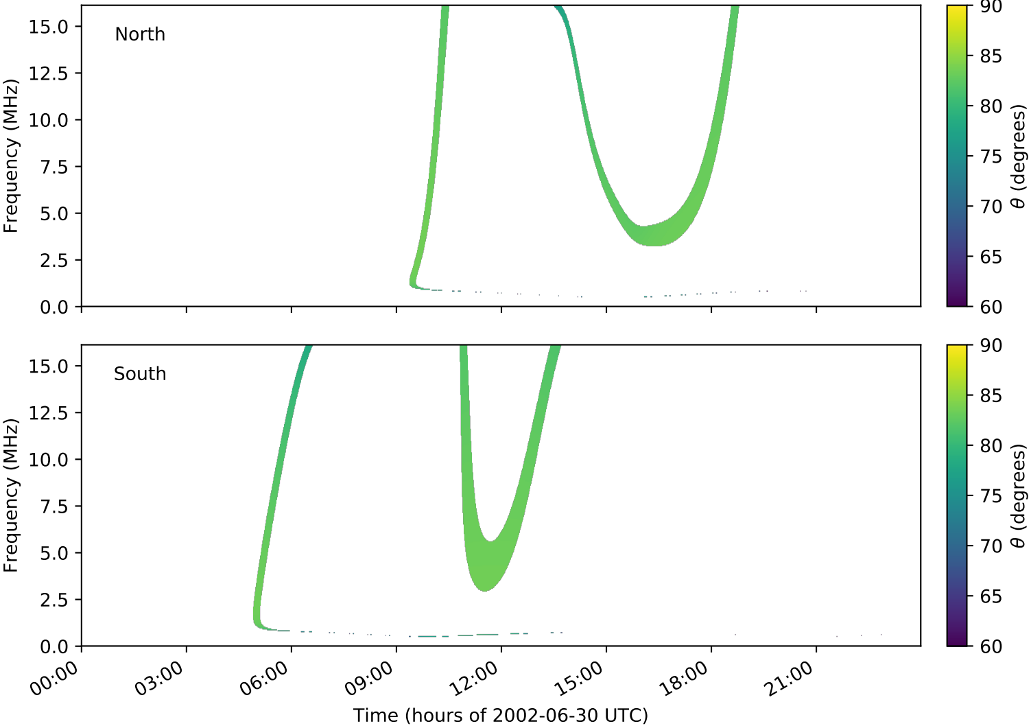
expres_cassini_jupiter_ganymede_isaac_lossc-wid1deg_3kev_20020630_v01.cdf
