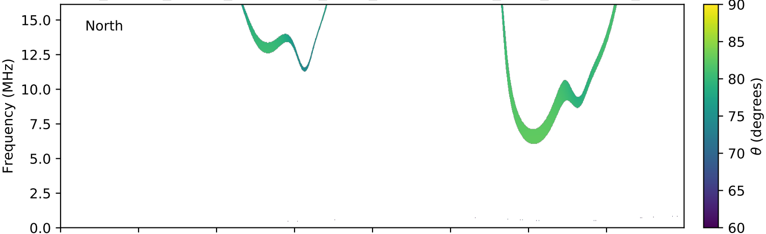
expres_cassini_jupiter_ganymede_isaac_lossc-wid1deg_3kev_20020625_v01.cdf
