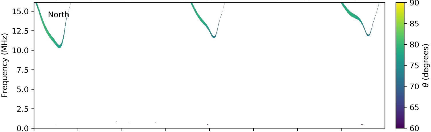
expres_cassini_jupiter_ganymede_isaac_lossc-wid1deg_3kev_20020624_v01.cdf
