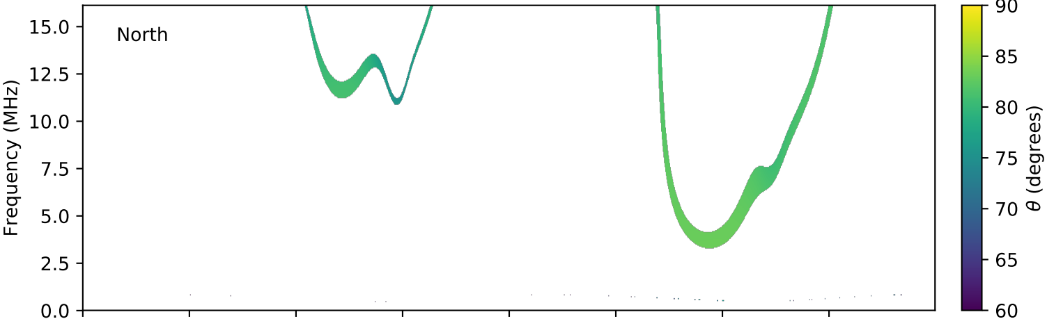
expres_cassini_jupiter_ganymede_isaac_lossc-wid1deg_3kev_20020618_v01.cdf
