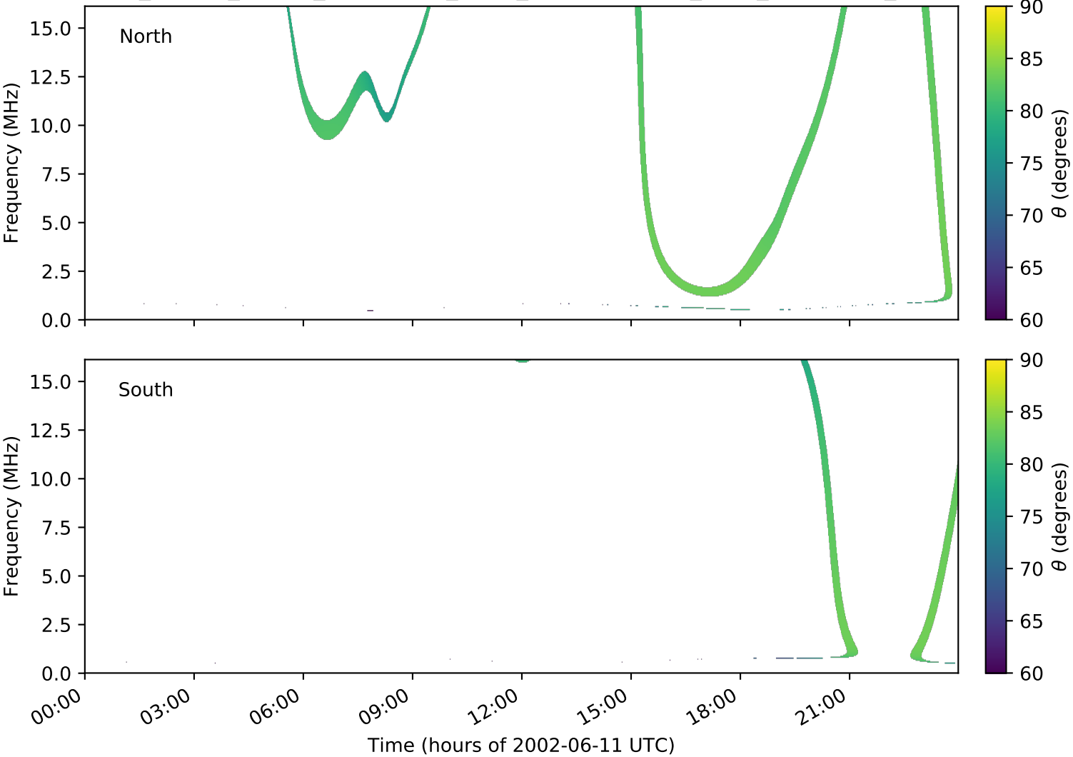
expres_cassini_jupiter_ganymede_isaac_lossc-wid1deg_3kev_20020611_v01.cdf
