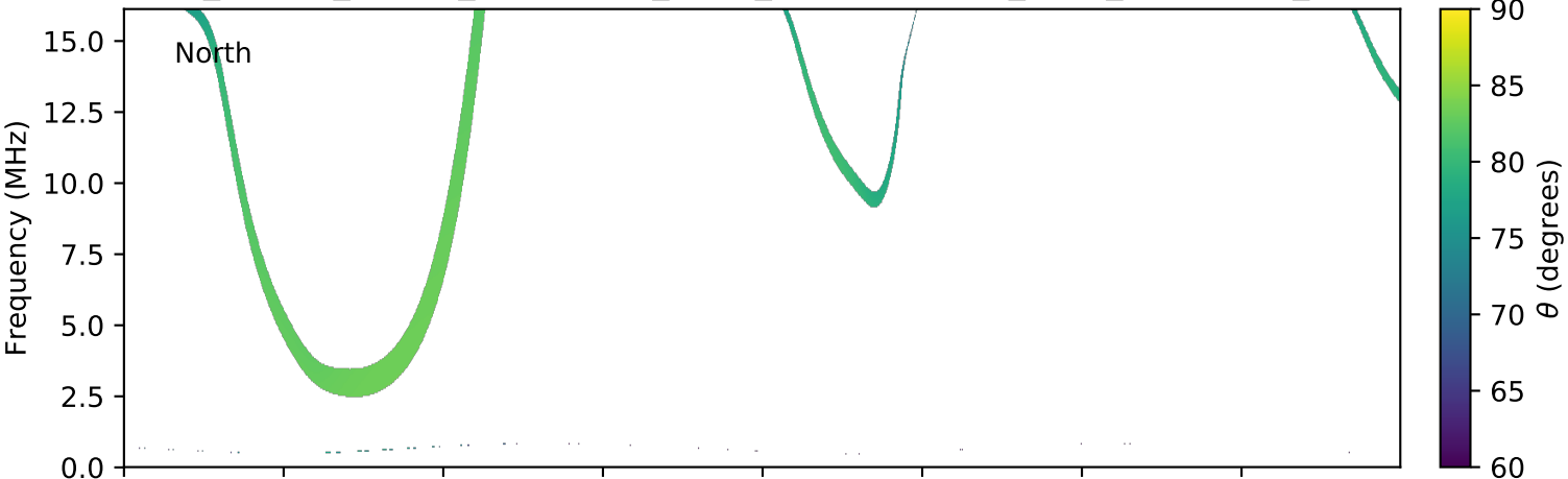
expres_cassini_jupiter_ganymede_isaac_lossc-wid1deg_3kev_20020609_v01.cdf
