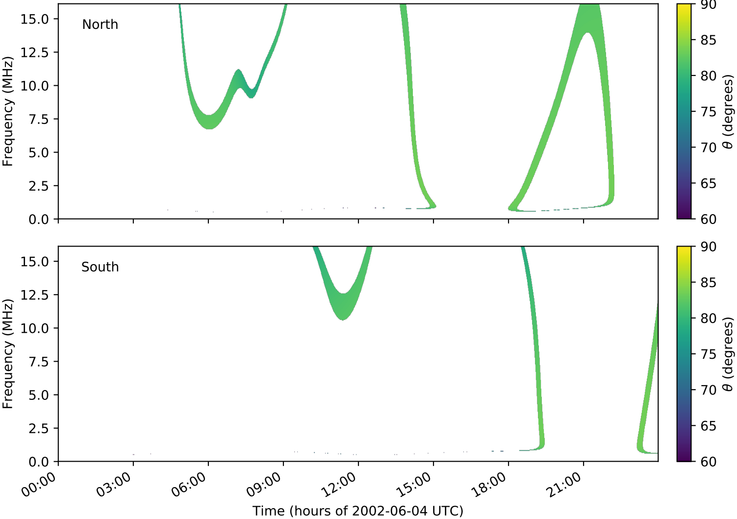
expres_cassini_jupiter_ganymede_isaac_lossc-wid1deg_3kev_20020604_v01.cdf
