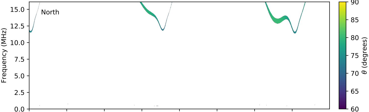
expres_cassini_jupiter_ganymede_isaac_lossc-wid1deg_3kev_20020603_v01.cdf
