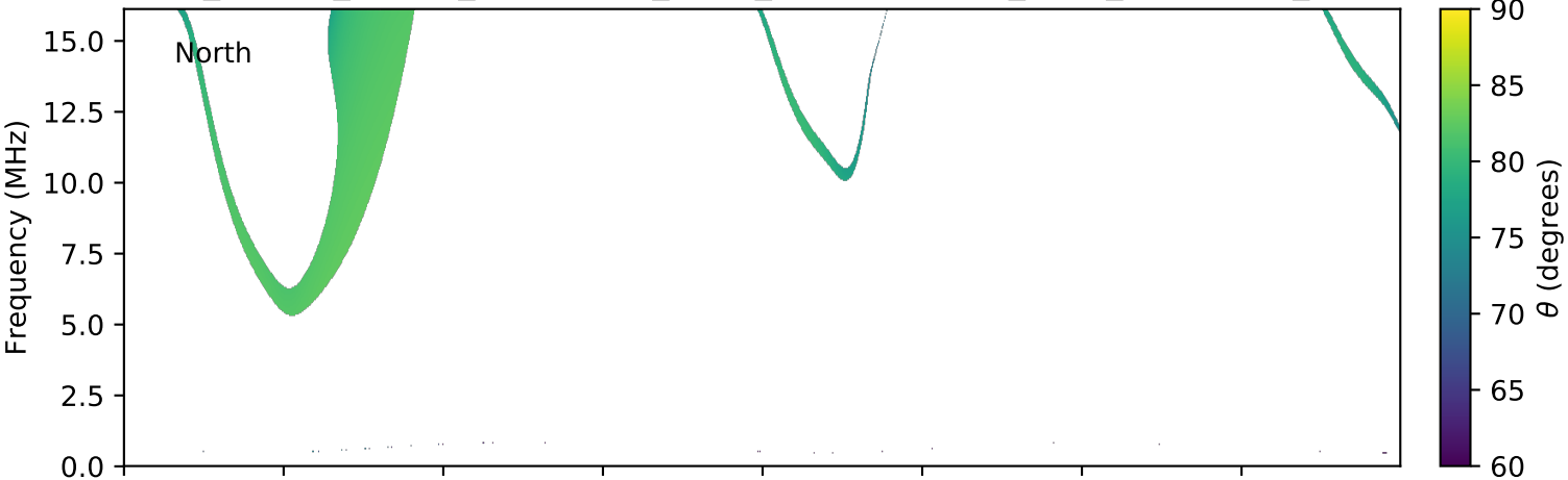
expres_cassini_jupiter_ganymede_isaac_lossc-wid1deg_3kev_20020602_v01.cdf
