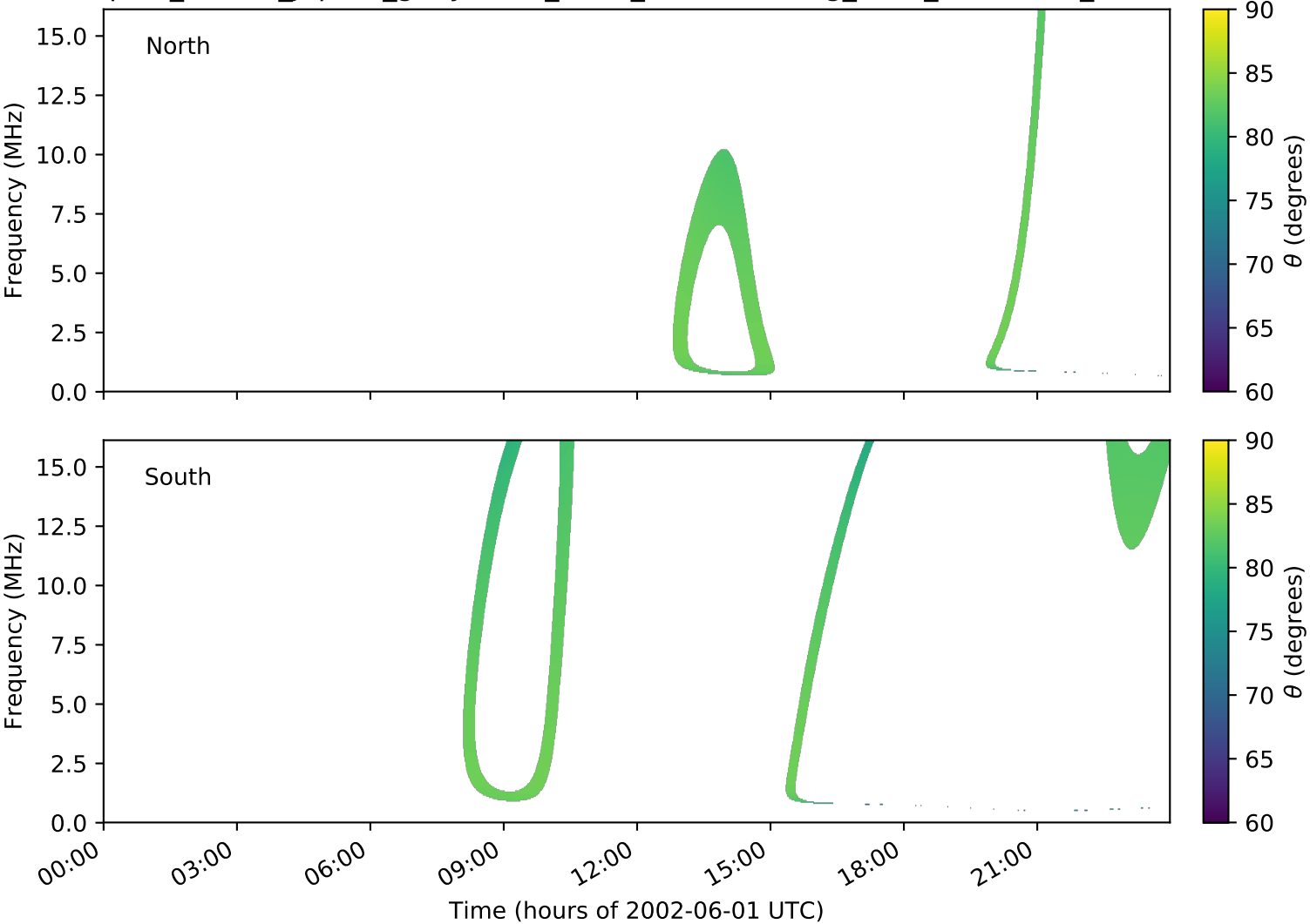
expres_cassini_jupiter_ganymede_isaac_lossc-wid1deg_3kev_20020601_v01.cdf
